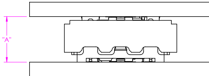
FIGURE 1 UDM6 MATED WITH UDF6
